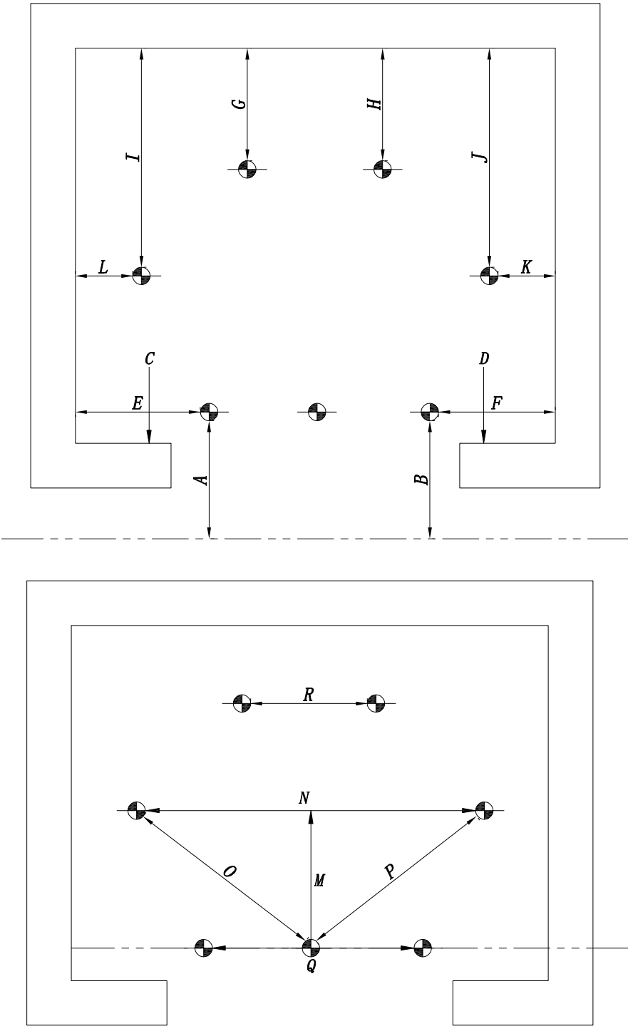
REAR COUNTERWEIGHT
