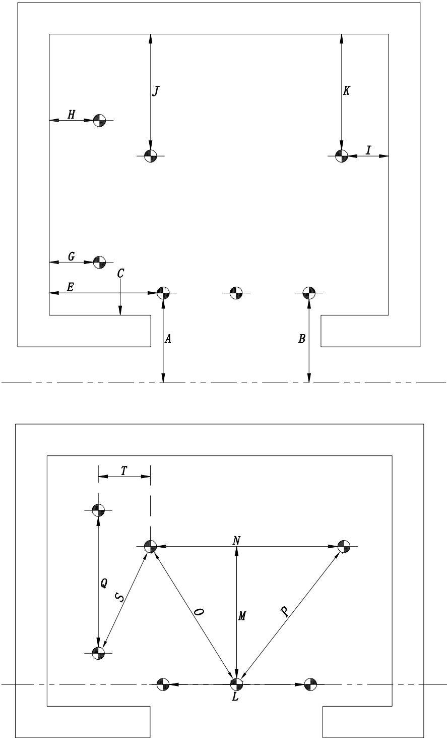
LEFT COUNTERWEIGHT
